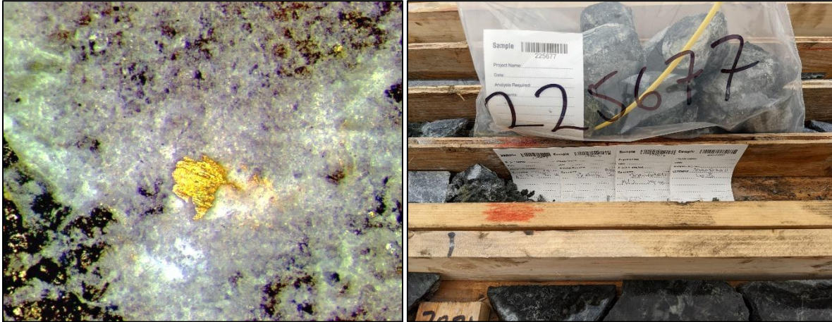
Figure 2. Visible gold occurrence MN22-05 70.2m. Gold grains range from <1mm to 3mm as irregular particles disseminated or along microfractures mainly within quartz and serpentine in listwanized peridotite. Gold was noted with fine to coarse-grained brecciated pyrite, chalcopyrite with pyrrhotite and galena. Field of view approximately 15mm. Right – core sample and QA/QC for visible gold interval 69.95-70.25m.
