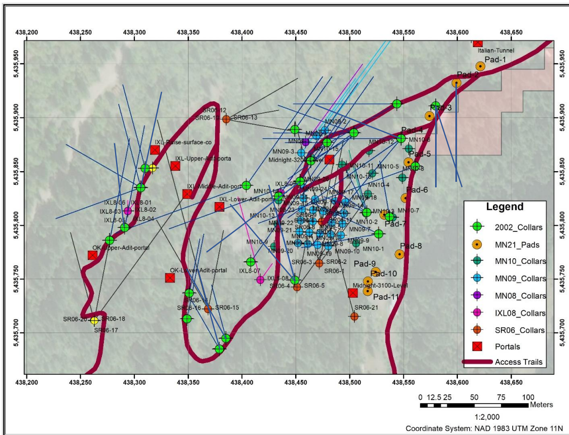
Figure 1. Location map of current and pending 2022, and post-2000 historical drilling on Midnight, IXL and OK mining claims and grants with mine portals and access trails. Current drilling at OK Upper Portal, IXL Lower Adit and northeast of Midnight 3100 and 3200 Portals.
